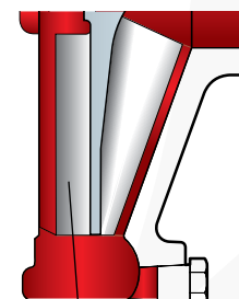
Back Pump-Out Vanes
